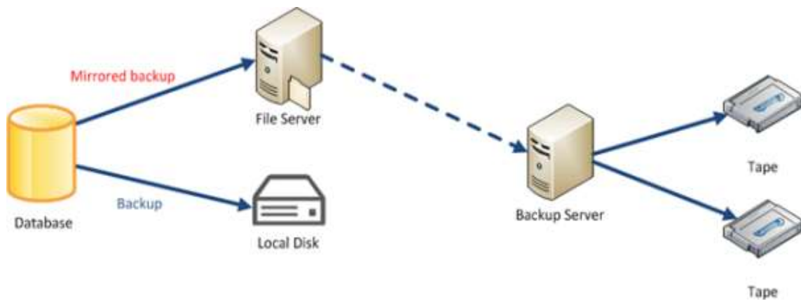
Figure 2.6. Database mirroring
