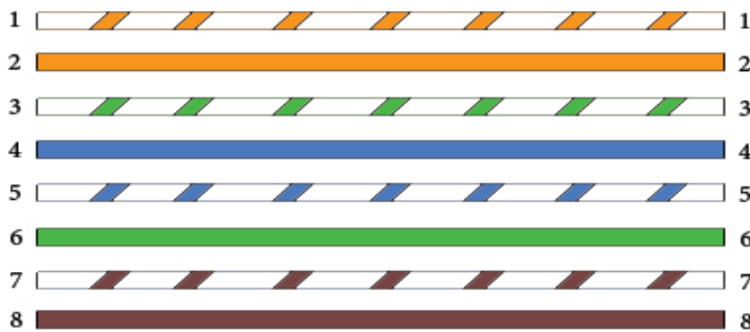
Straight Through Wiring Guide 568-B
